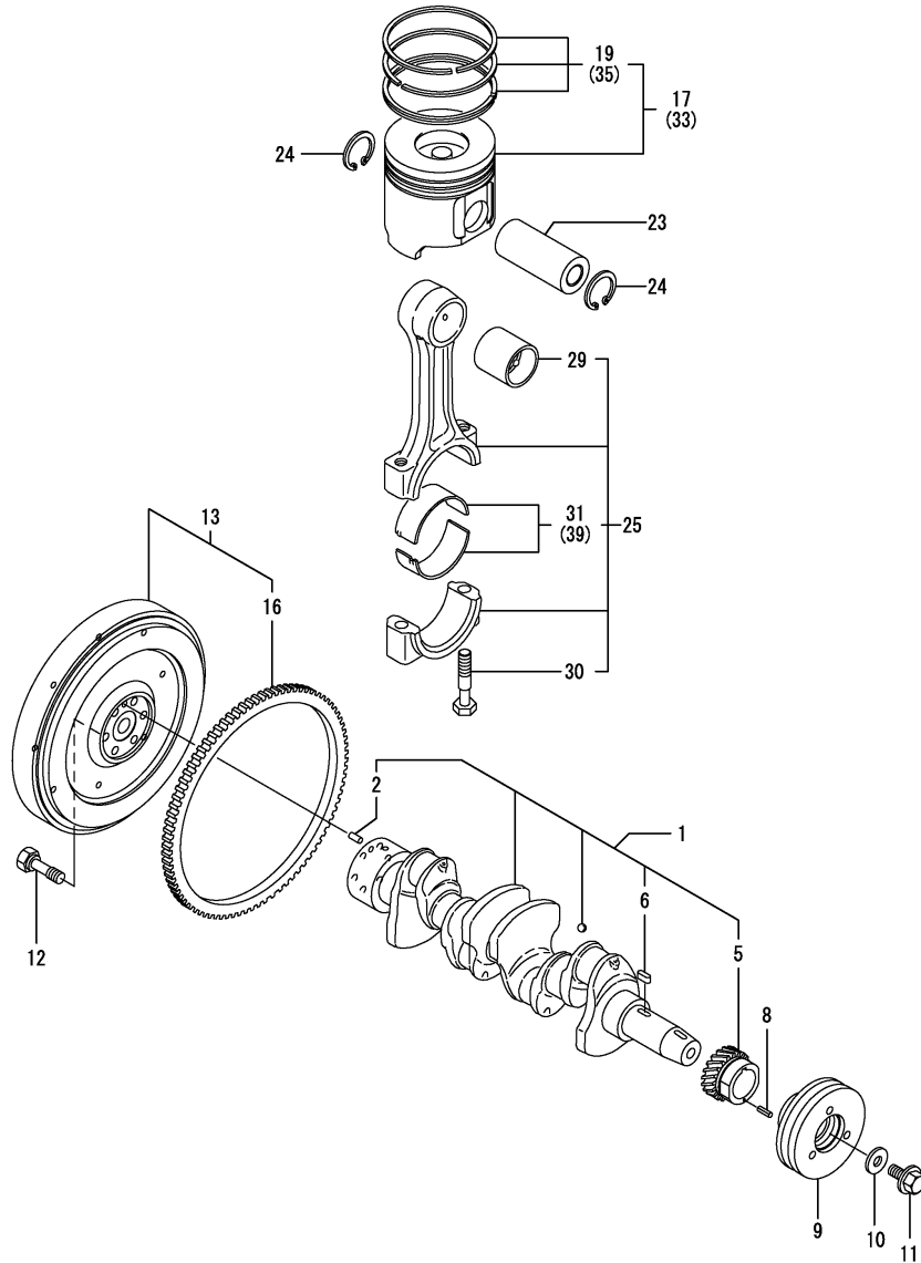
Fig.8. CRANKSHAFT & PISTON
