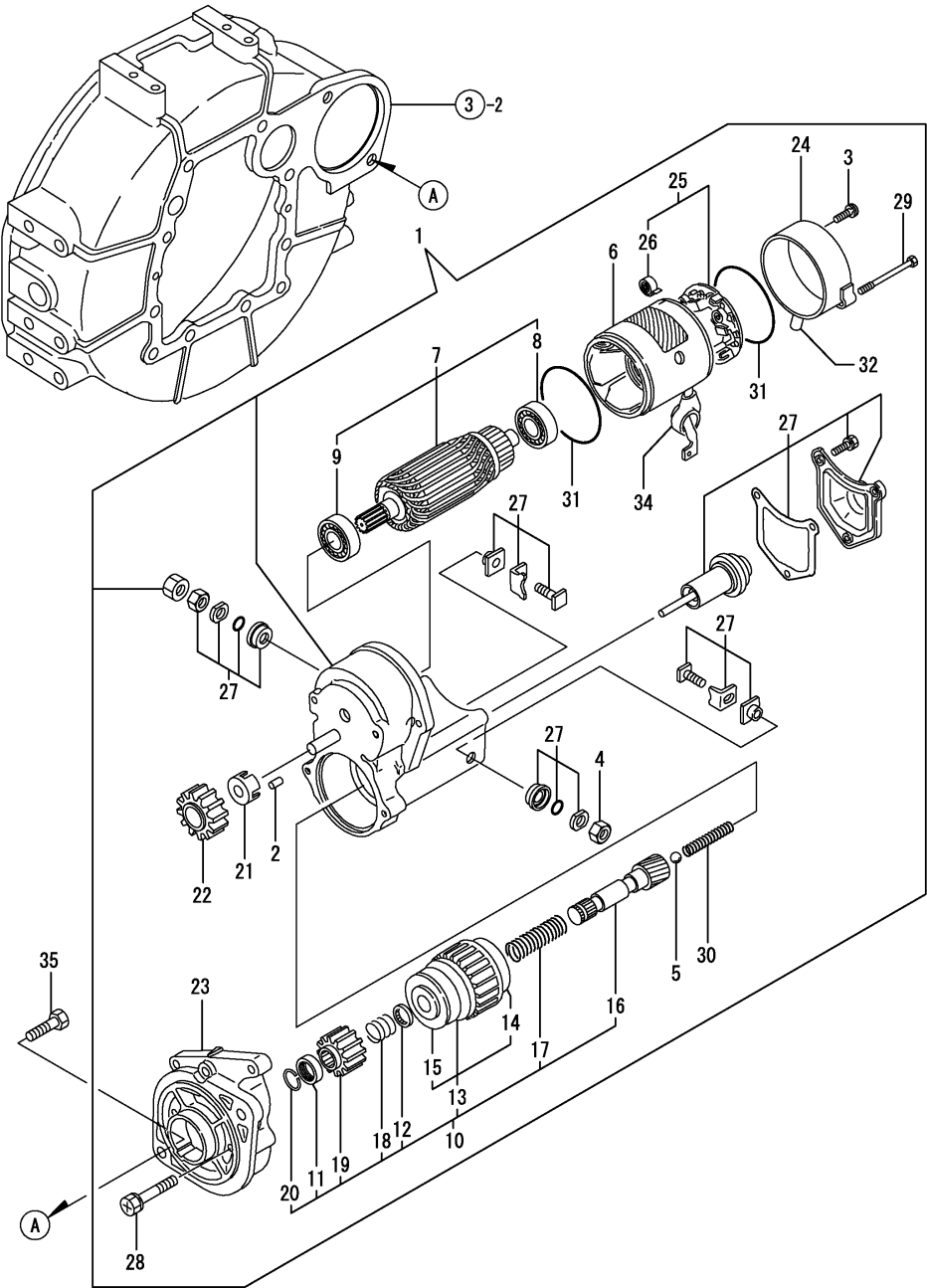
Fig.15. STARTING MOTOR
