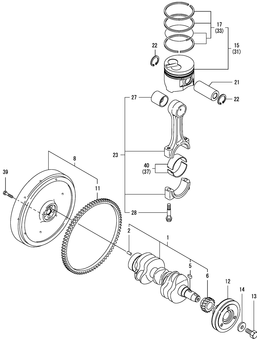
Fig.6. CRANKSHAFT & PISTON
