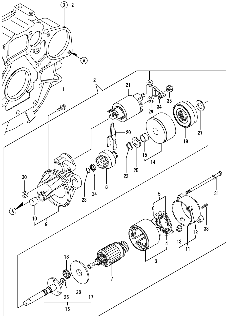
Fig.13. STARTING MOTOR
