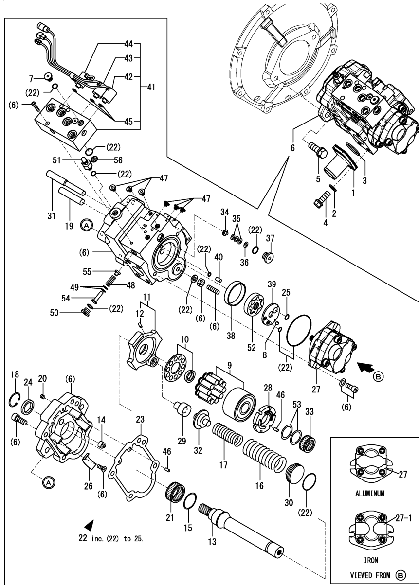
Fig.86. HYDRAULIC PUMP(ESS SPEC.)
