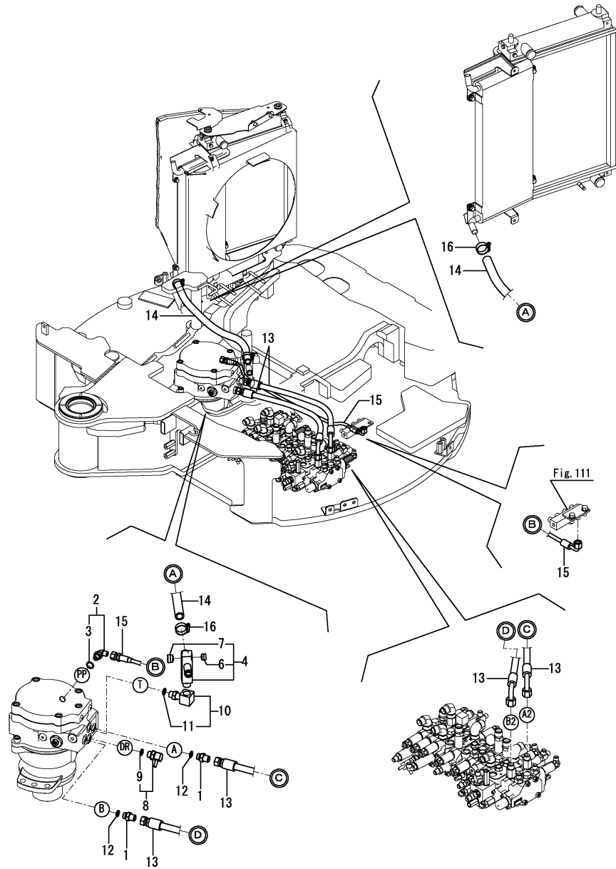
Fig.109. CONTROL VALVE - TURNING MOTOR
