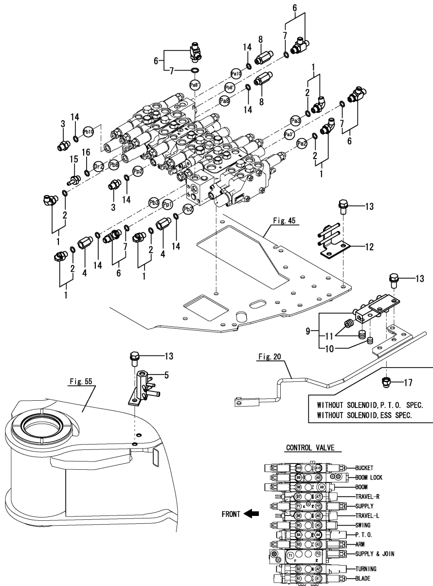
Fig.111. CONTROL VALVE(FITTING)(2)
