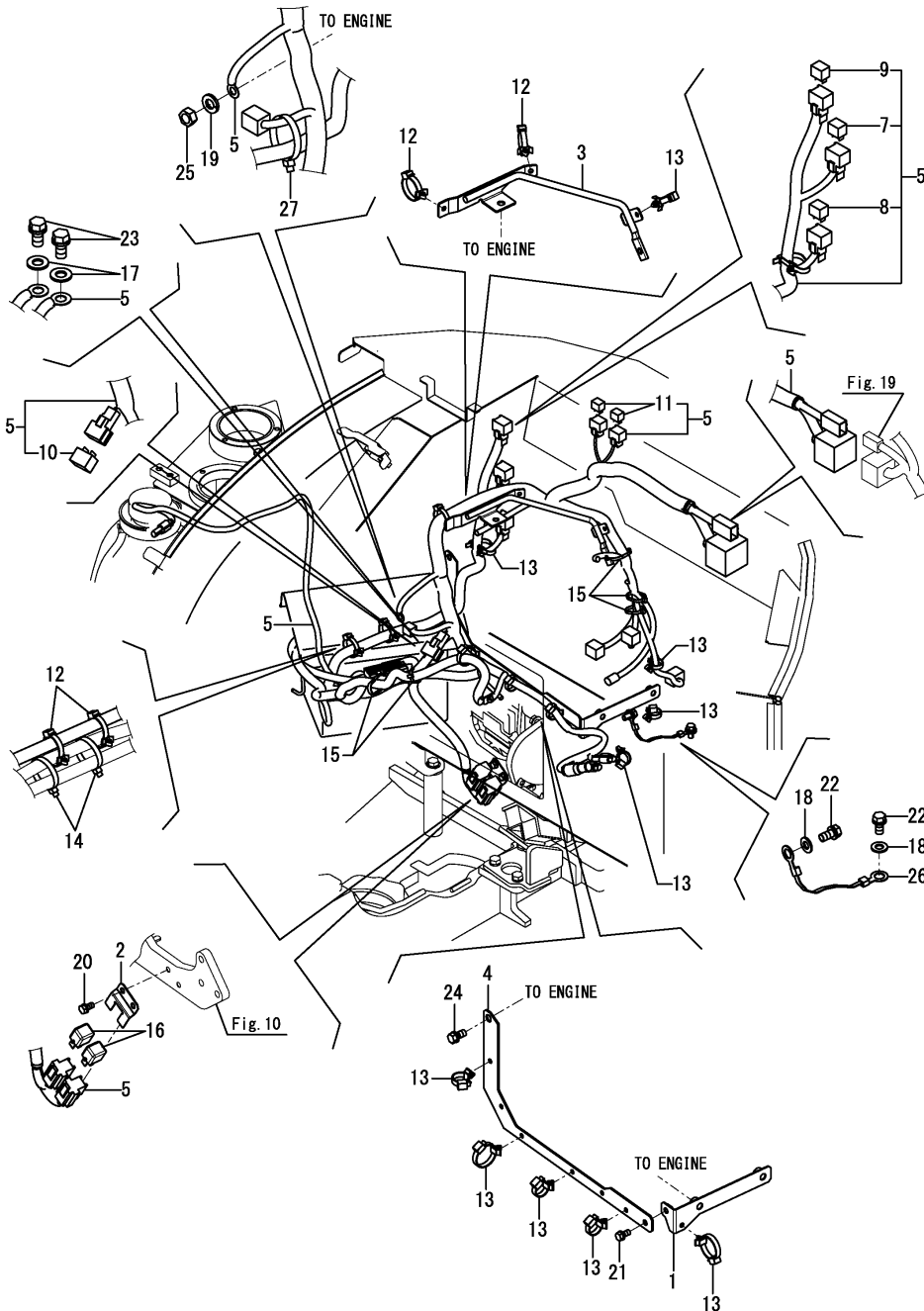
Fig.190. (17A)AROUND THE ENGINE(FROM M61126)
