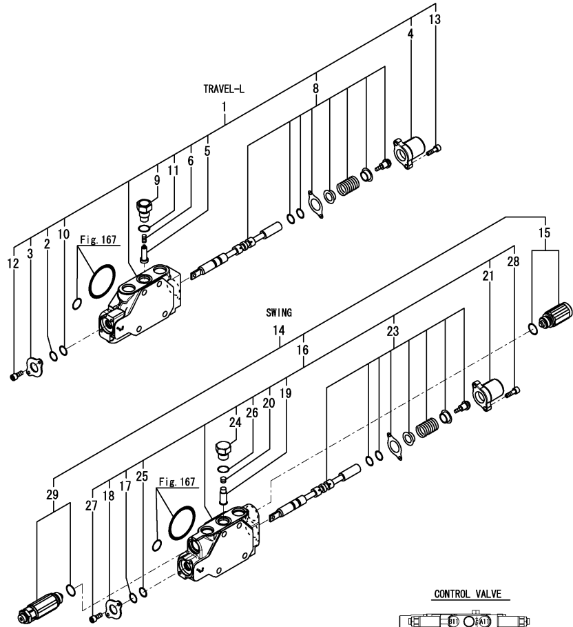
Fig.170. (101E)CONTROL VALVE(5/8)(ANGLE BLADE SPEC.)
