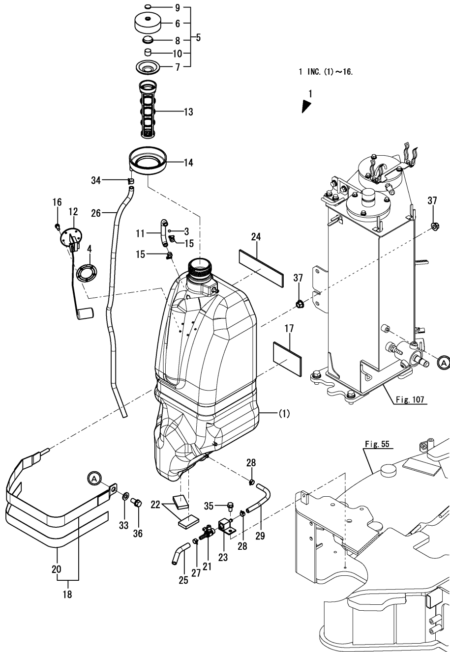
Fig.14. FUEL TANK
