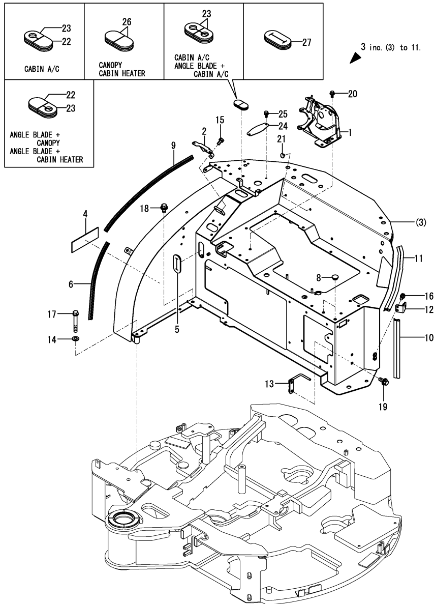
Fig.68. SEAT MOUNT
