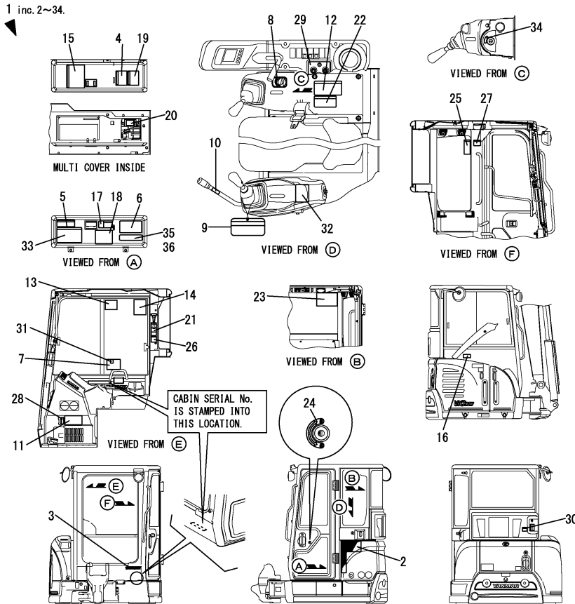
Fig.4. LABEL(CABIN)(TO MAF000)
