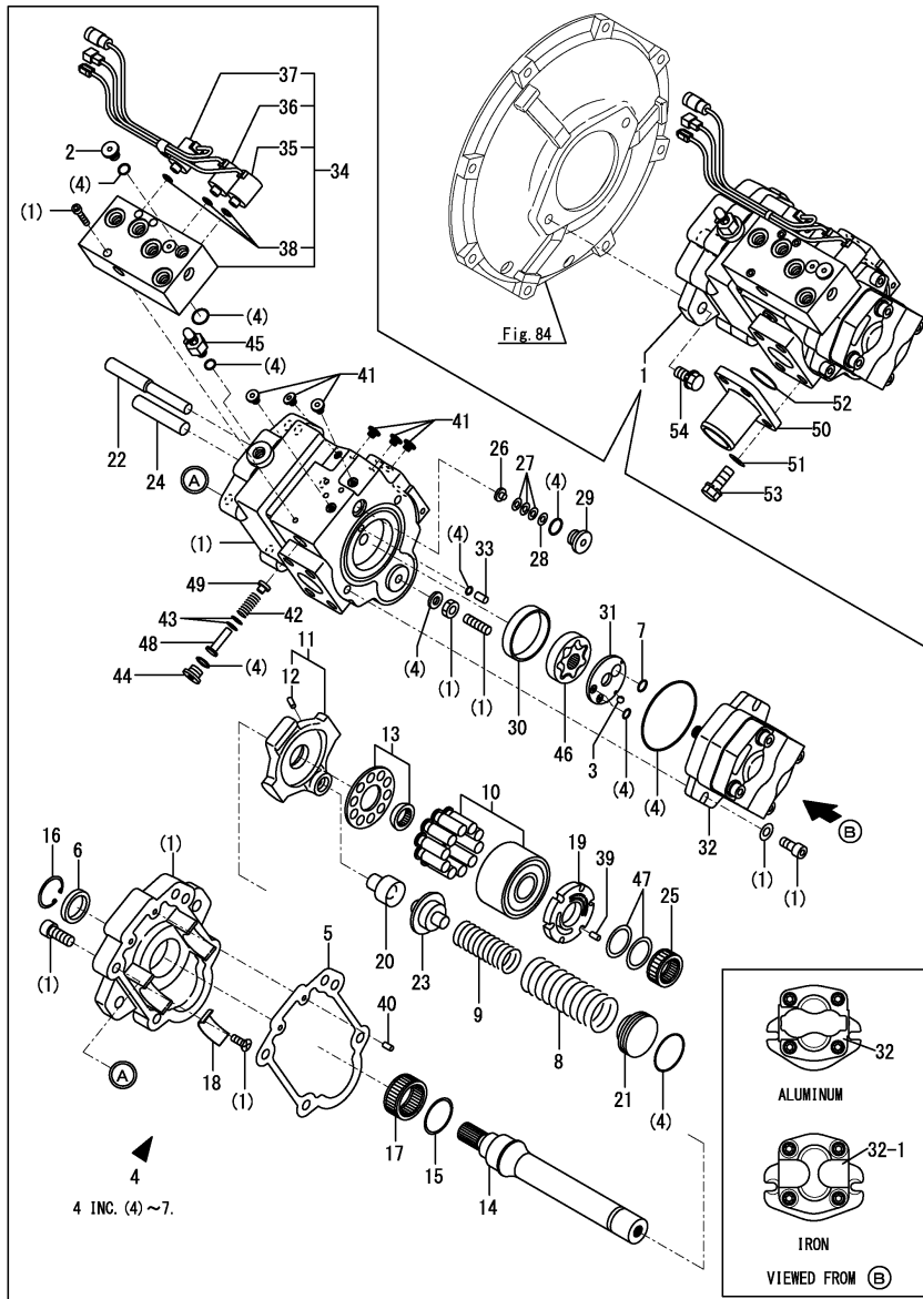
Fig.85. HYDRAULIC PUMP(QUIK COUPLER SPEC.)
