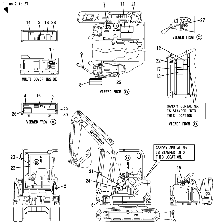
Fig.200. (3A)LABEL(CANOPY)(FROM MAF001)
