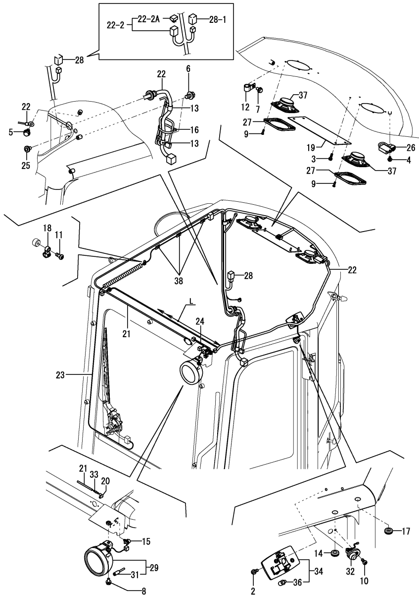
Fig.146. (80G)CABIN(ELECTRIC PARTS)
