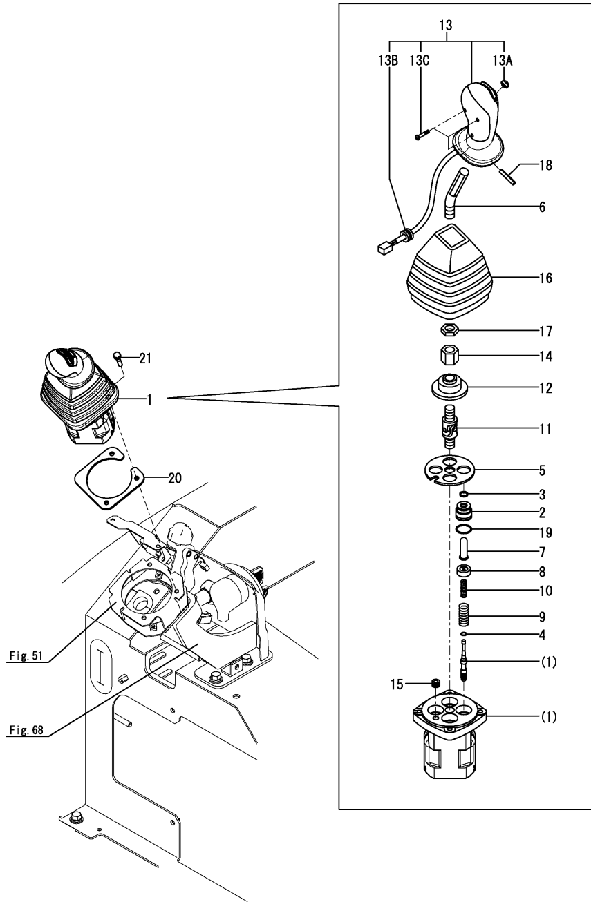
Fig.102. REMOTE CONTROL VALVE(RIGHT)(TO MAH583)
