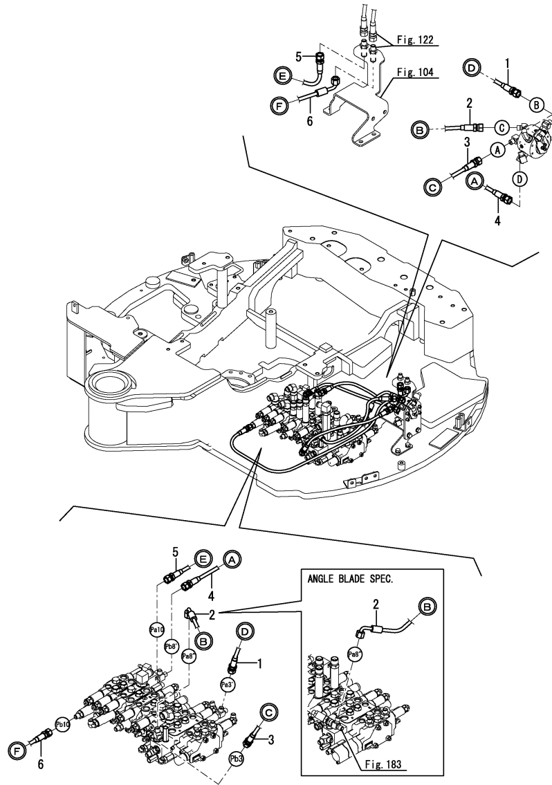
Fig.123. CONTROL PIPING(2)
