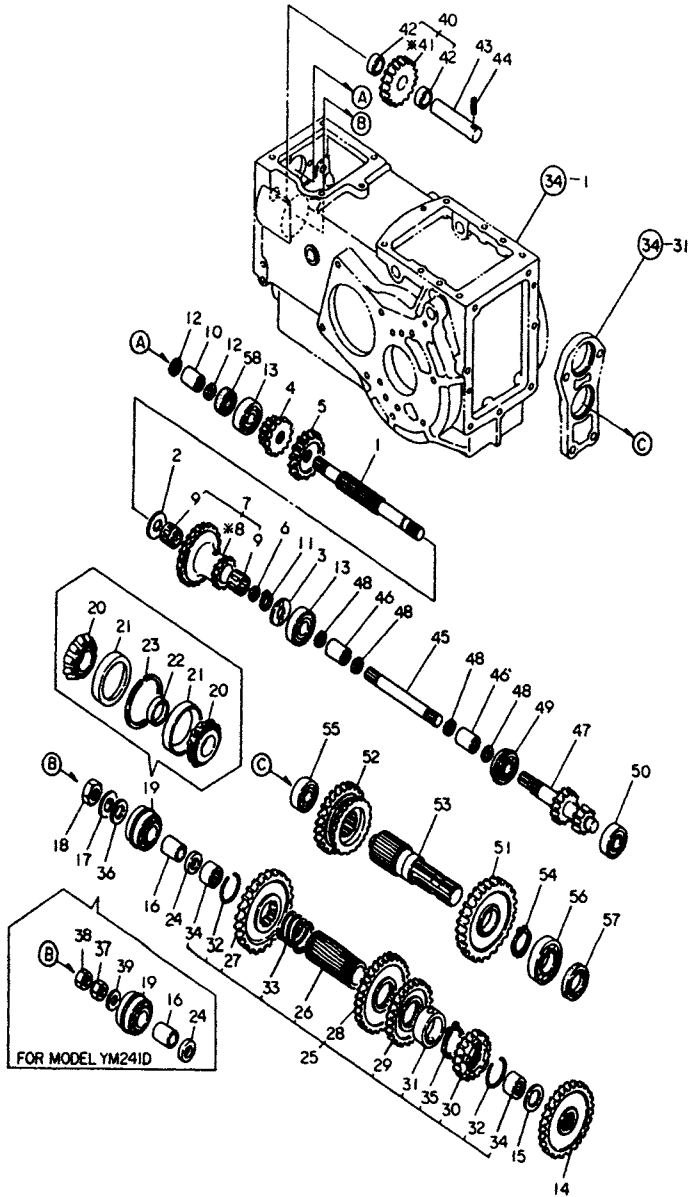
Fig. 36 TRANSMISSION GEARS
