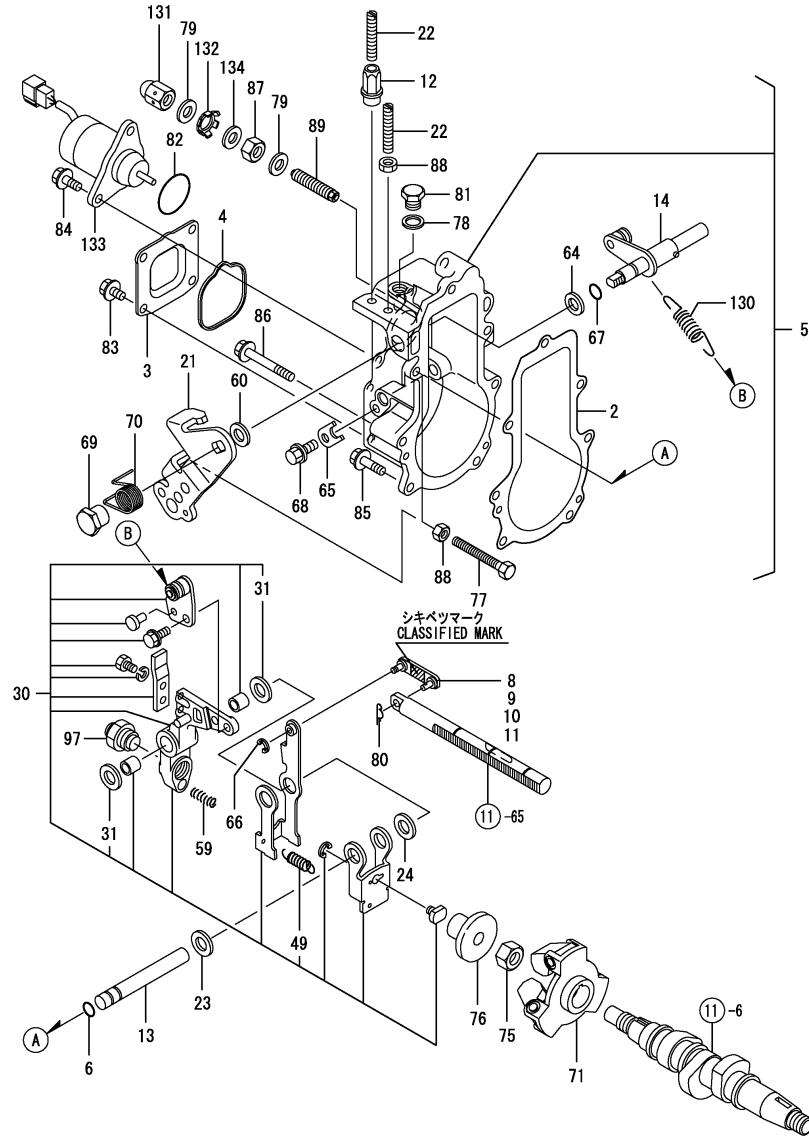
Fig.12. GOVERNOR
