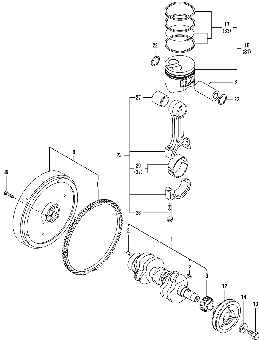
Fig.8. CRANKSHAFT & PISTON
