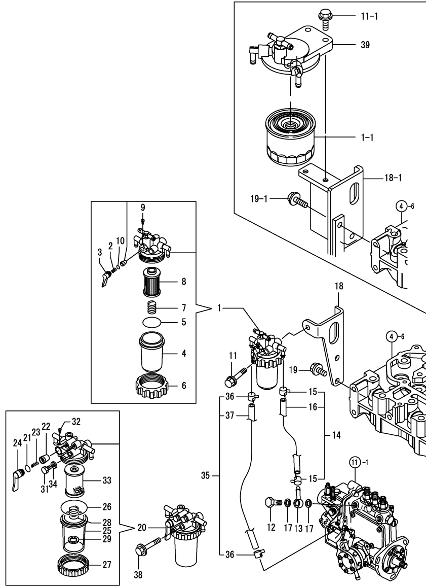
Fig.14. FUEL LINE
