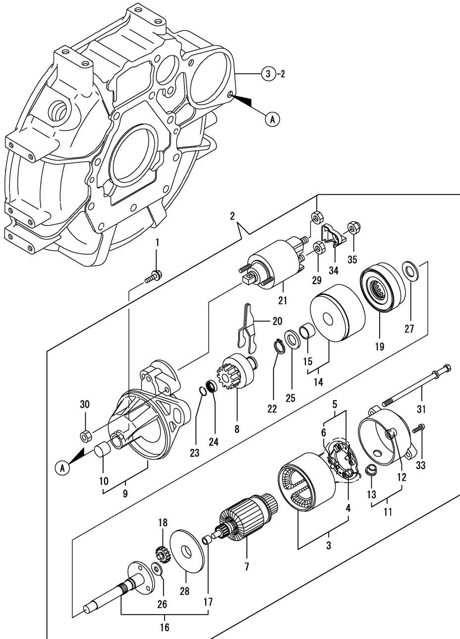
Fig.15. STARTING MOTOR
