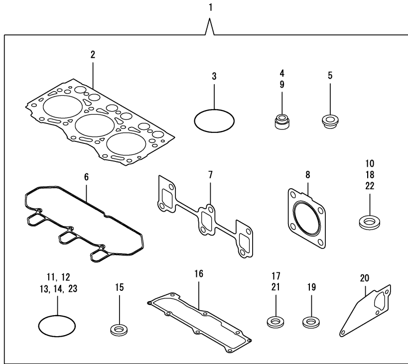
Fig.17. GASKET SET & TOOLS
