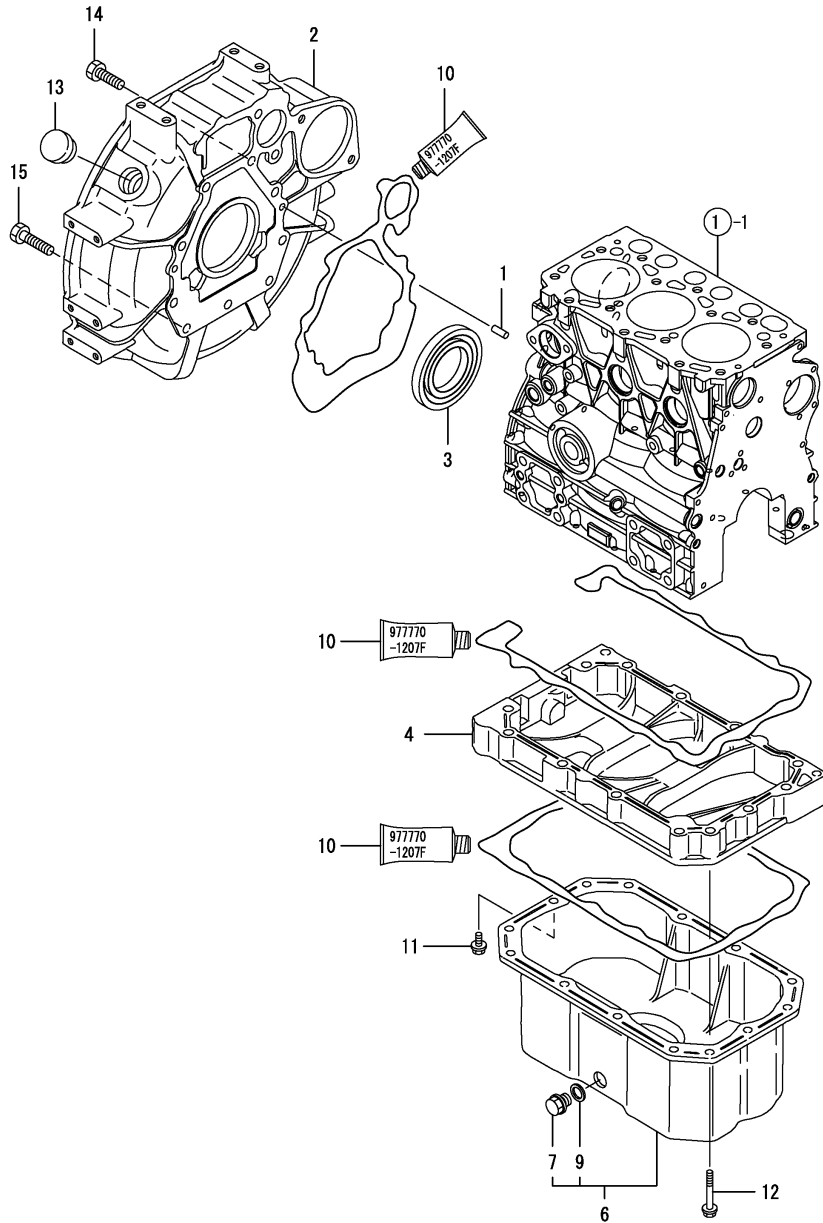
Fig.3. FLYWHEEL HOUSING & OIL SUMP
