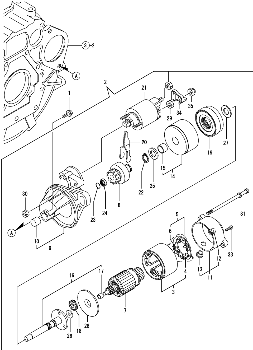
Fig.15. STARTING MOTOR
