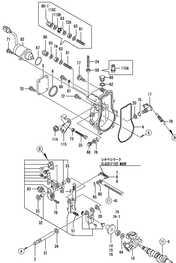
Fig.12. GOVERNOR
