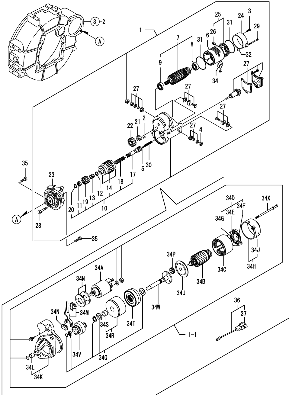
Fig.15. STARTING MOTOR
