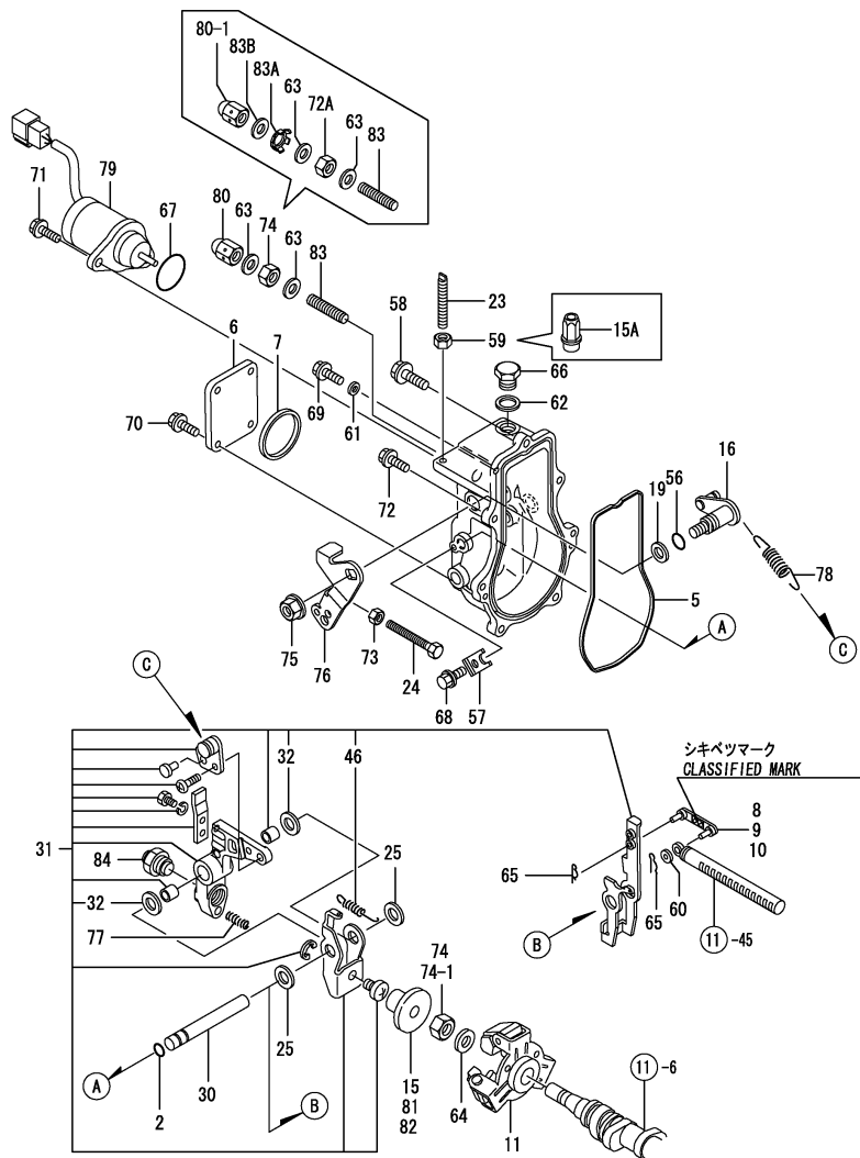
Fig.12. GOVERNOR
