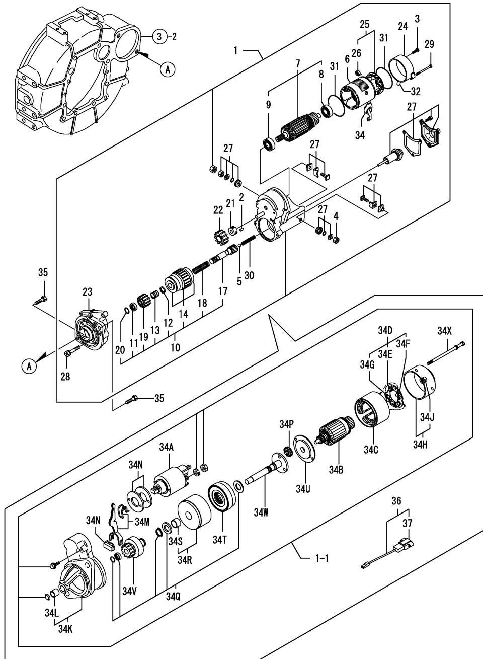
Fig.15. STARTING MOTOR
