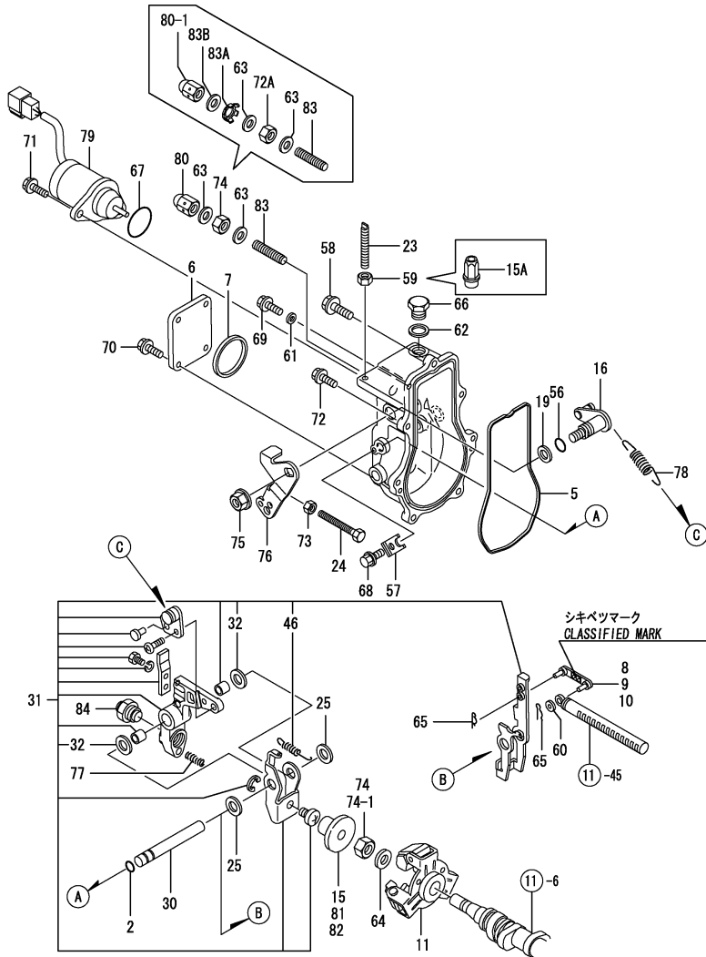
Fig.12. GOVERNOR
