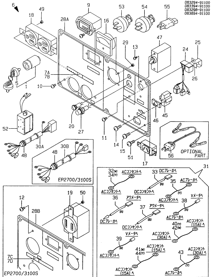
Fig.16. PANEL(EP1700/2000/2700/3100S)
