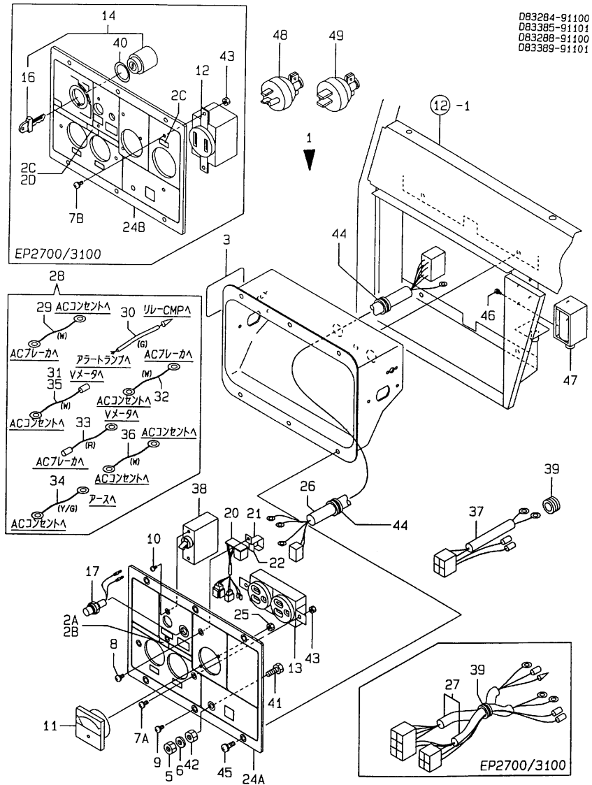
Fig.15. PANEL(EP1700/2000/2700/3100)
