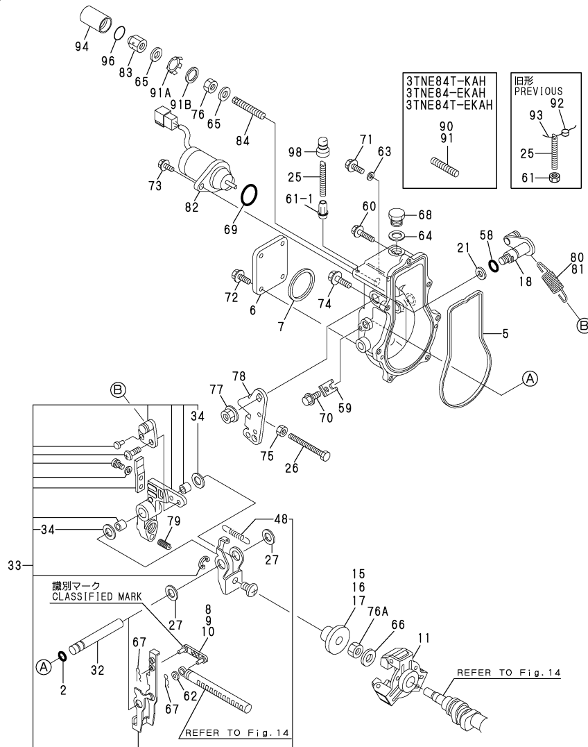
Fig.15. GOVERNOR
