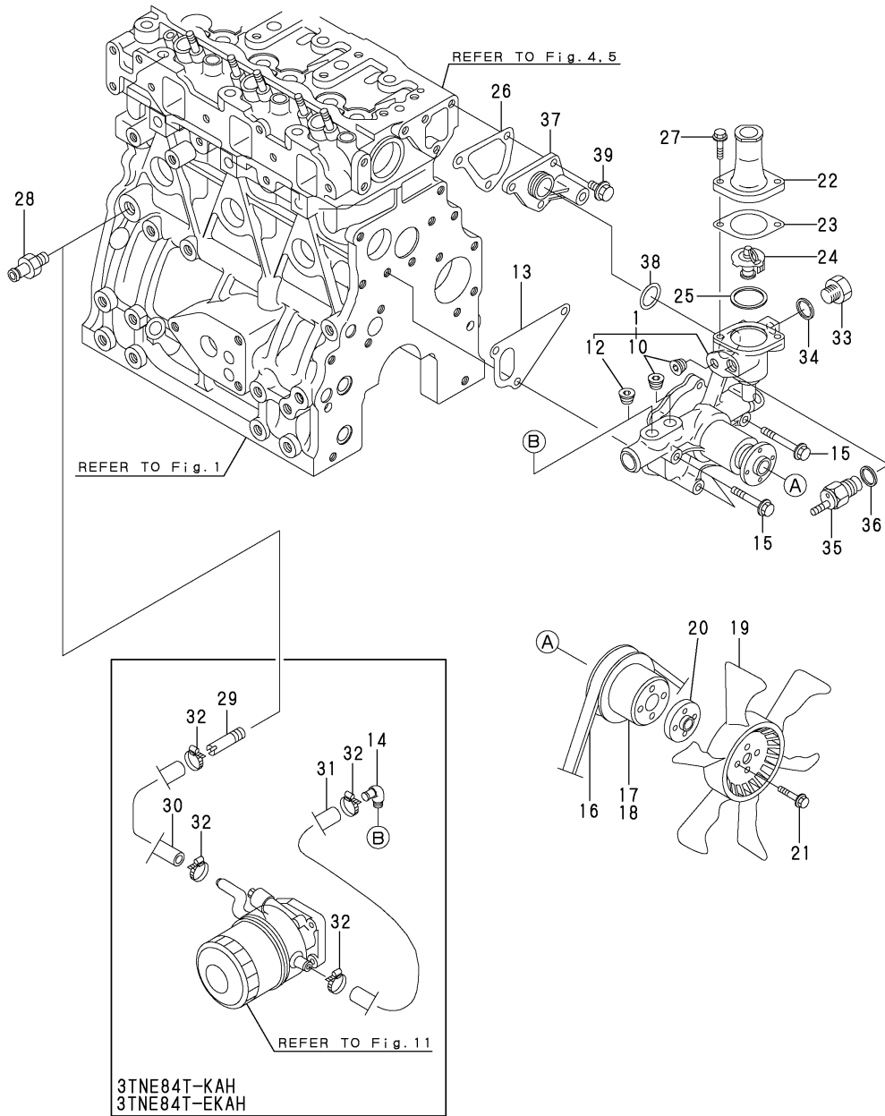
Fig.13. COOLING WATER SYSTEM
